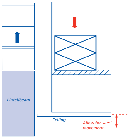
As built
