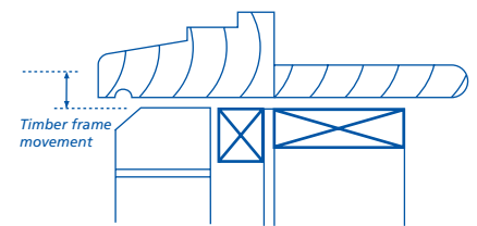
After movement
