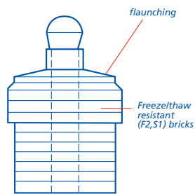
CHIMNEY DETAIL WITH BRICK CAPPING
