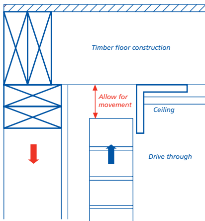
As Built
