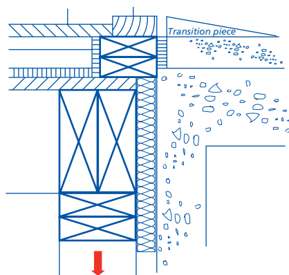
As built
