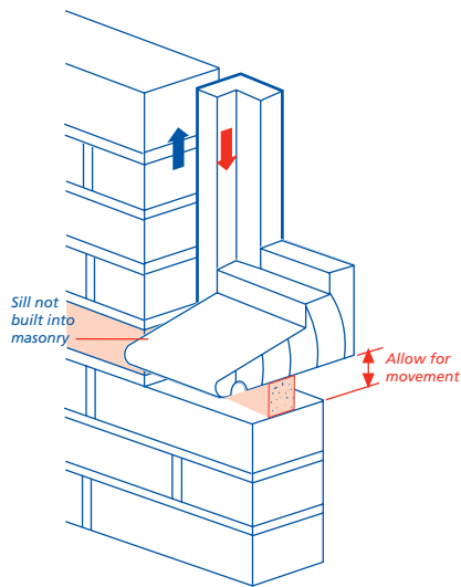
Normal reveal
