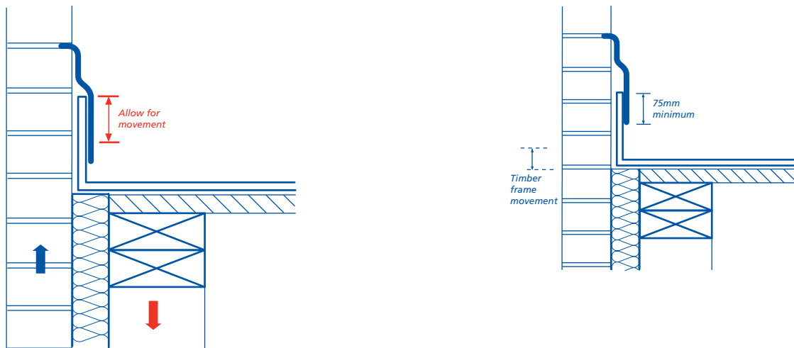
After movement
